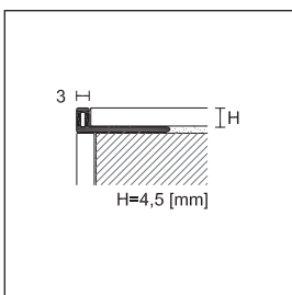
PV/8 PVC bege cinza
